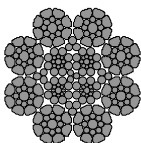
Section / Cross section Cable / Rope type : A
