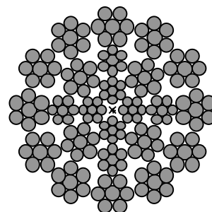
Section / Cross section Cable / Rope type : F and Y
